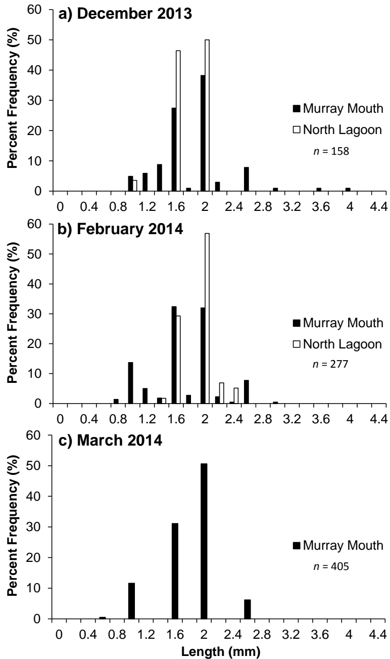
Figure 11. Size-frequency distribution histograms for Arthritica helmsi for each sampling occasion in the Murray Mouth and North Lagoon regions.
