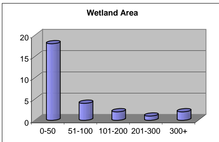
Figure 13-1. Wetland area.
